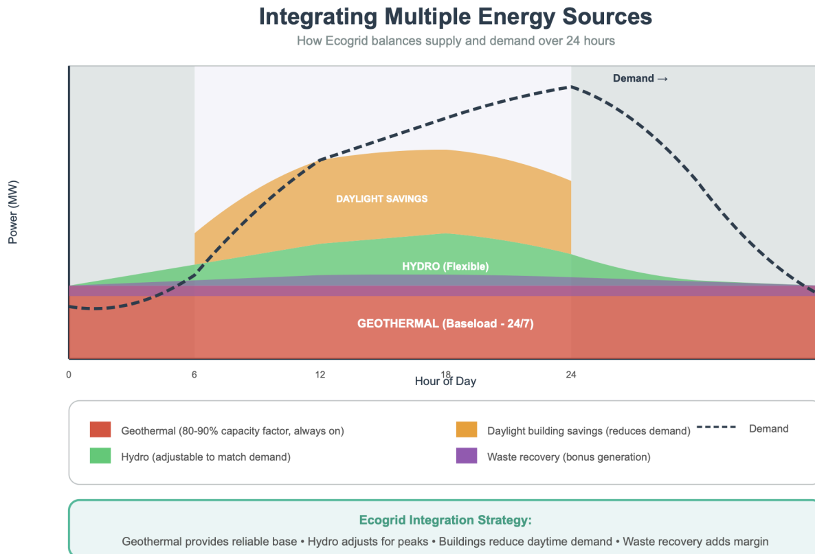
Figure 12.1: Integrating Multiple Energy Sources Over 24 Hours
