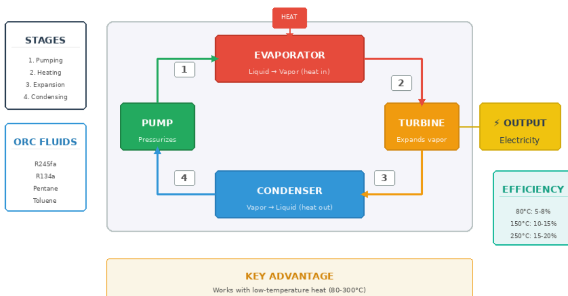
Figure 7.2: Organic Rankine Cycle (ORC) for Heat Recovery
